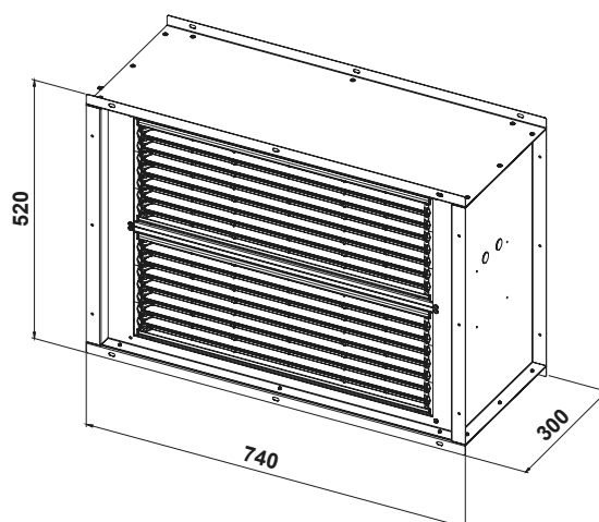
CDS.C2
